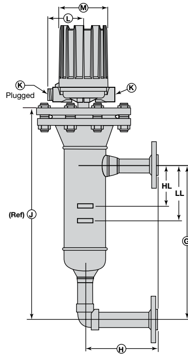
Figure 16 Flanged Side/Side
