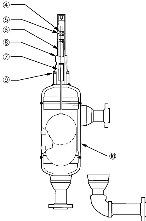
Figure 19 Sealed Cage Models B35, C35, G35
