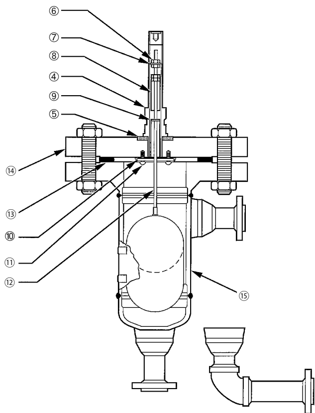
Figure 20 Flanged Cage Models B3F, G3F, K3F
