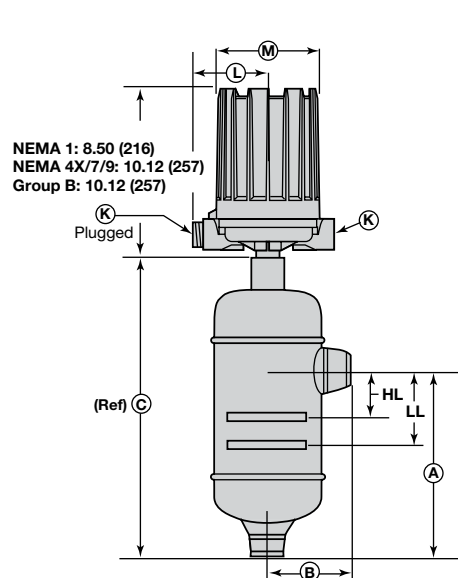
Figure 12 Threaded & Socket Weld Upper Side/Bottom
