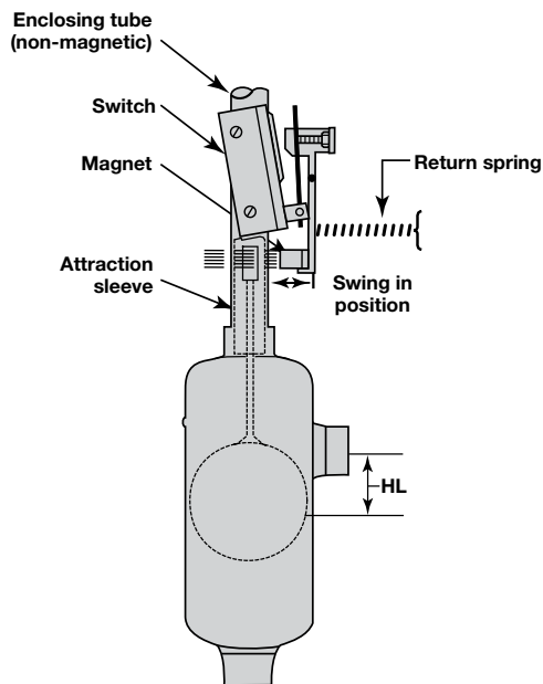
Figure 1 Switch Tripped
